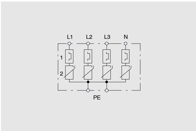
Block diagram of V25-B+C/4-G
