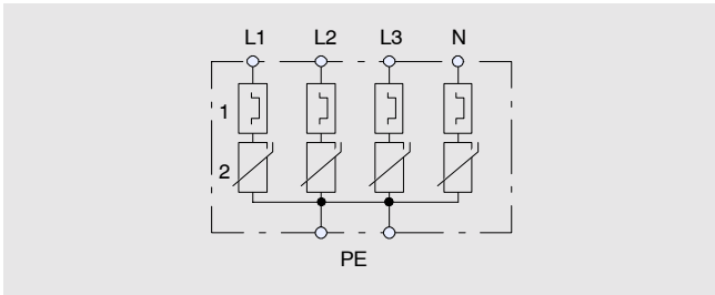
Block diagram of V 25-B+C/4
