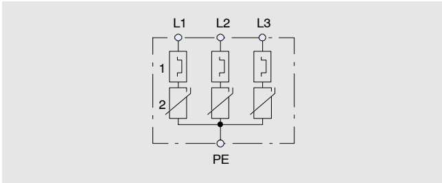
Block diagram of V 25-B+C/3
