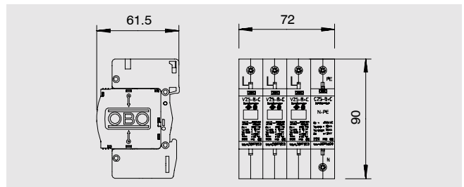
Dimension drawing
