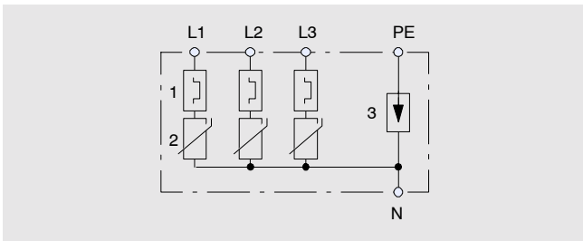
Block diagram of V 25-B+C/3+NPE
